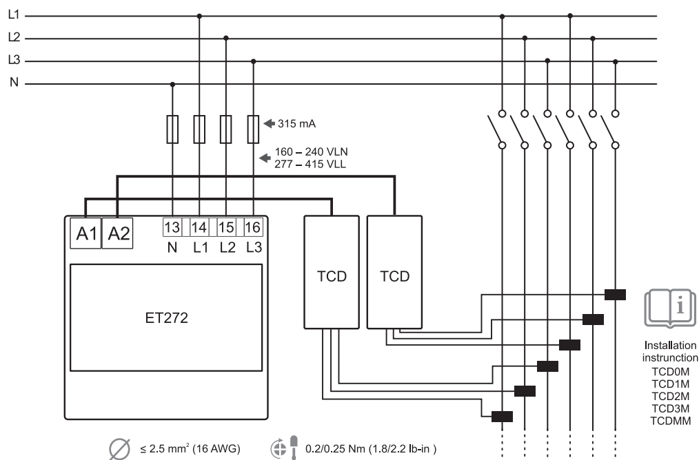
Fig. 2 Voltage and current input connection diagram
