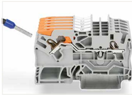
Insert fine-stranded conductors with ferrules via push-in termination.
