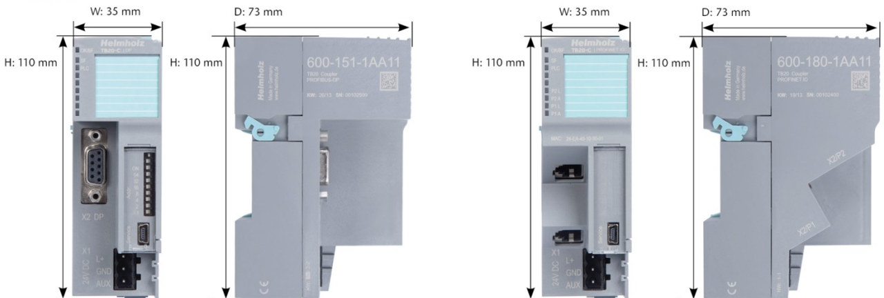
Bus Coupler
