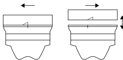
Fig. 7 Open/close
